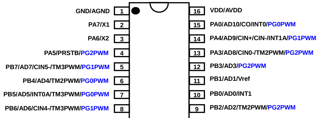
PMS132/PMS132B-S16B (SOP16B-150mil)
