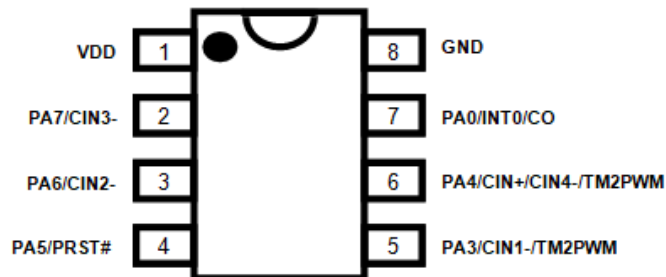
PMS150C-S08 (SOP8-150mil)
